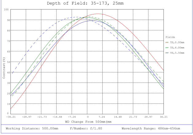
#35-173, 25mm, f/1.8 Cr Series Fixed Focal Length Lens, Depth of Field Plot, 500mm Working Distance, f1.8
