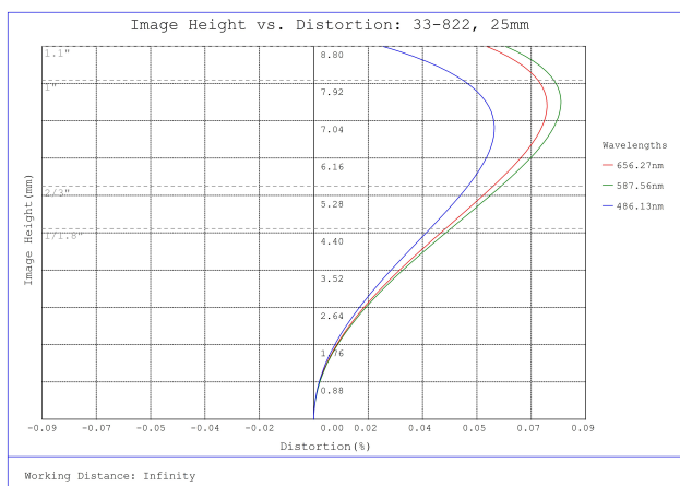
#33-822, 25mm f/2.0, HPI Series Fixed Focal Length Lens, Distortion Plot
