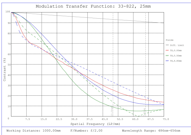
#33-822, 25mm f/2.0, HPI Series Fixed Focal Length Lens, Modulated Transfer Function (MTF) Plot, 1000mm Working Distance, f2
