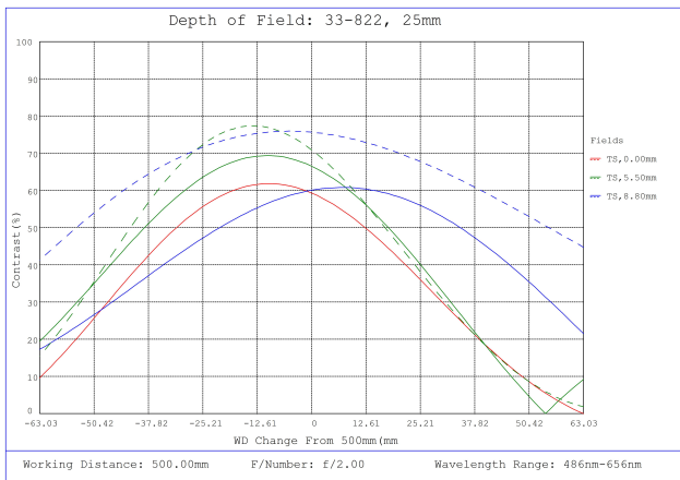
#33-822, 25mm f/2.0, HPI Series Fixed Focal Length Lens, Depth of Field Plot, 500mm Working Distance, f2
