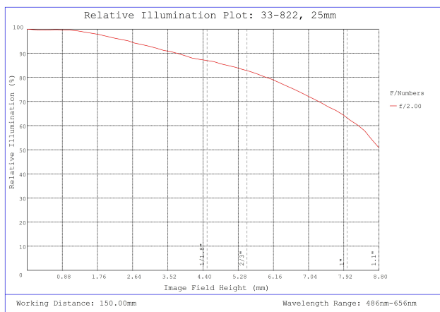
#33-822, 25mm f/2.0, HPI Series Fixed Focal Length Lens, Relative Illumination Plot
