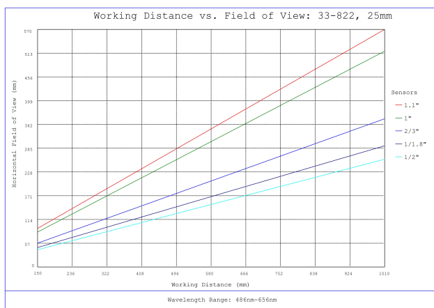
#33-822, 25mm f/2.0, HPI Series Fixed Focal Length Lens, Working Distance versus Field of View Plot
