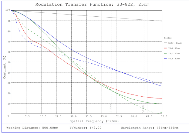
#33-822, 25mm f/2.0, HPI Series Fixed Focal Length Lens, Modulated Transfer Function (MTF) Plot, 500mm Working Distance, f2
