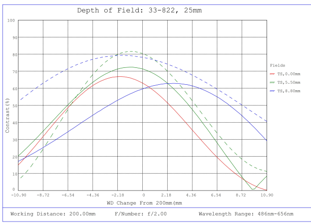
#33-822, 25mm f/2.0, HPI Series Fixed Focal Length Lens, Depth of Field Plot, 200mm Working Distance, f2
