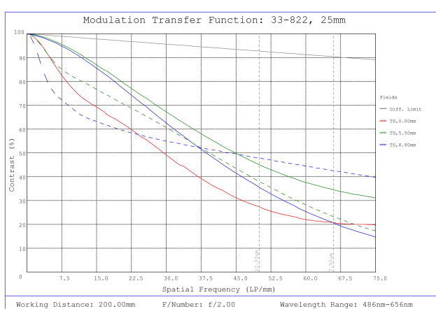
#33-822, 25mm f/2.0, HPI Series Fixed Focal Length Lens, Modulated Transfer Function (MTF) Plot, 200mm Working Distance, f2
