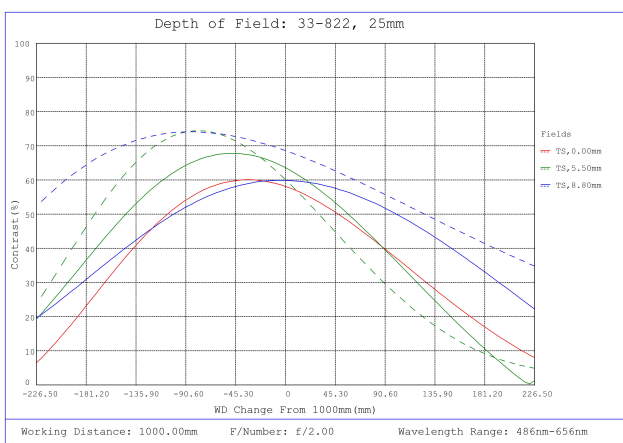
#33-822, 25mm f/2.0, HPI Series Fixed Focal Length Lens, Depth of Field Plot, 1000mm Working Distance, f2
