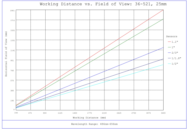
#36-521, 25mm f/4.0, HPr Series Fixed Focal Length Lens, Working Distance versus Field of View Plot
