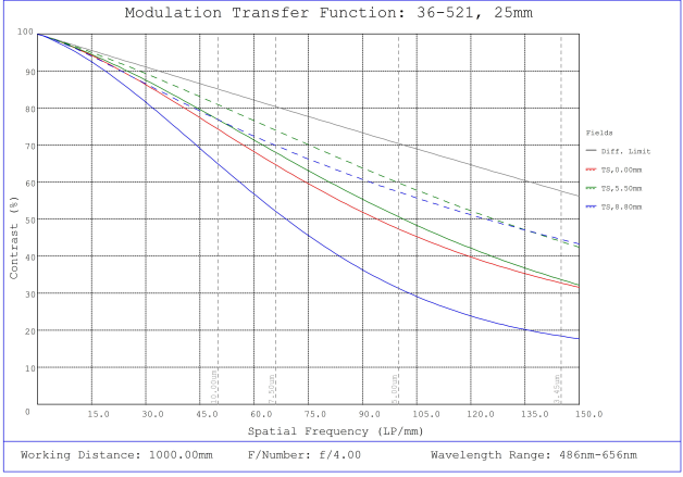
#36-521, 25mm f/4.0, HPr Series Fixed Focal Length Lens, Modulated Transfer Function (MTF) Plot, 1000mm Working Distance, f4
