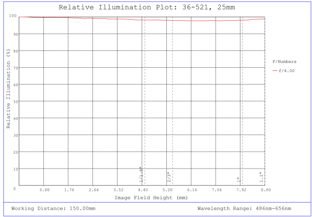
#36-521, 25mm f/4.0, HPr Series Fixed Focal Length Lens, Relative Illumination Plot
