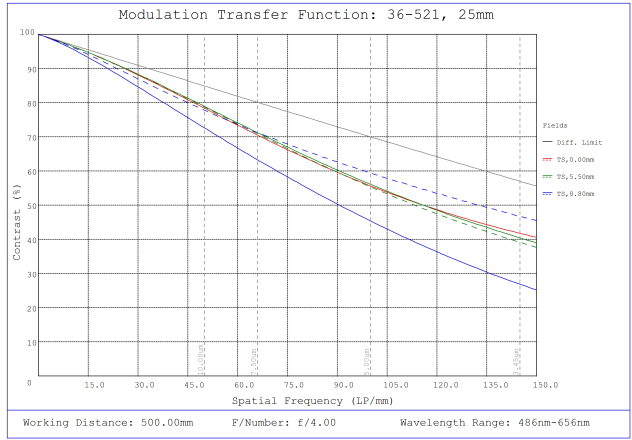
#36-521, 25mm f/4.0, HPr Series Fixed Focal Length Lens, Modulated Transfer Function (MTF) Plot, 500mm Working Distance, f4
