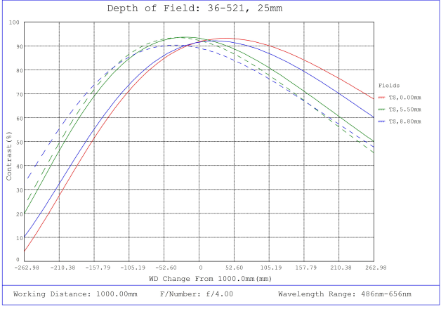
#36-521, 25mm f/4.0, HPr Series Fixed Focal Length Lens, Depth of Field Plot, 1000mm Working Distance, f4
