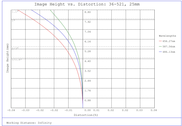
#36-521, 25mm f/4.0, HPr Series Fixed Focal Length Lens, Distortion Plot
