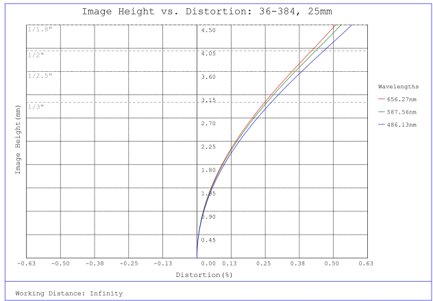
#36-384, 25mm FL f/2.5, Rugged Blue Series M12 Lens, Distortion Plot
