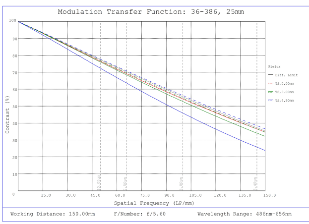
#36-386, 25mm FL f/5.6, Rugged Blue Series M12 Lens, Modulated Transfer Function (MTF) Plot, 150mm Working Distance, f5.6
