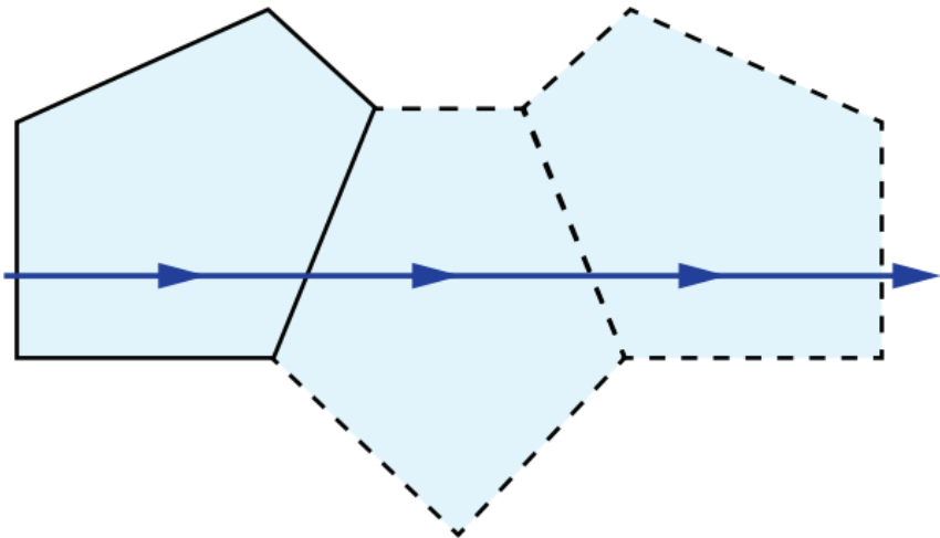
Penta Prism Tunnel Diagram
