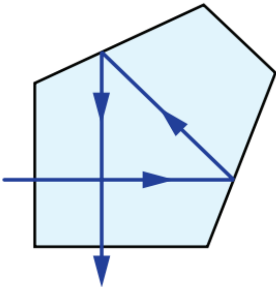
Penta Prism Ray Path
