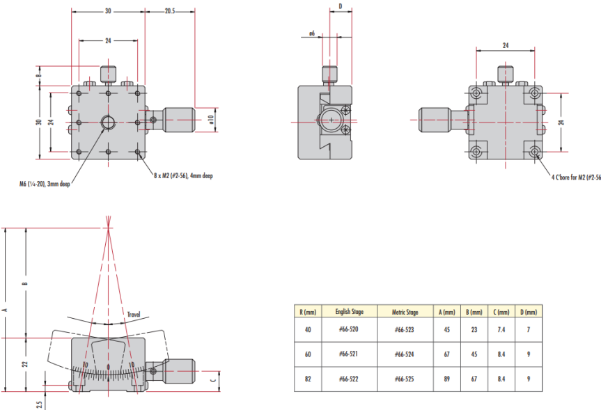
30mm Goniometers
