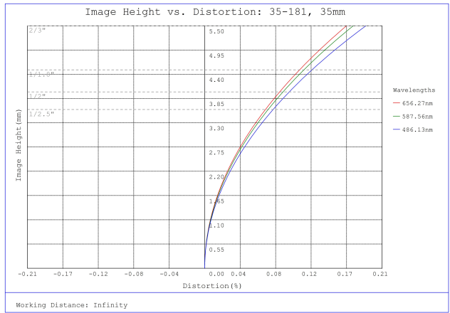
#35-181, 35mm, f/1.65 Cr Series Fixed Focal Length Lens, Distortion Plot
