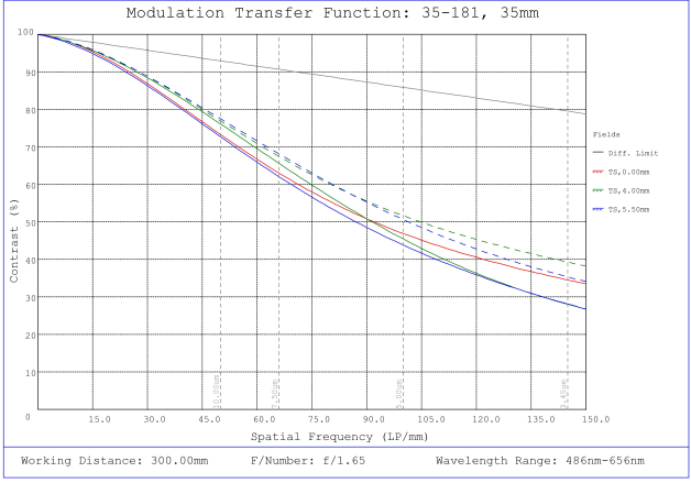
#35-181, 35mm, f/1.65 Cr Series Fixed Focal Length Lens, Modulated Transfer Function (MTF) Plot, 300mm Working Distance, f1.6
