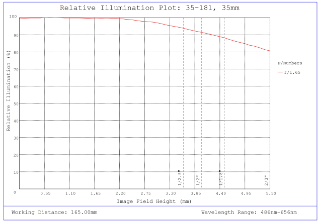
#35-181, 35mm, f/1.65 Cr Series Fixed Focal Length Lens, Relative Illumination Plot
