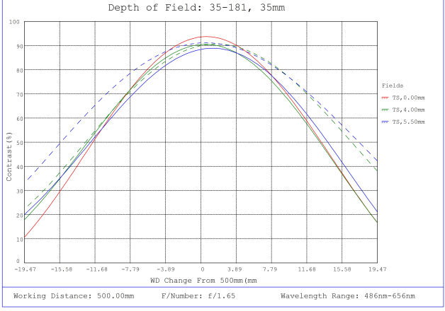
#35-181, 35mm, f/1.65 Cr Series Fixed Focal Length Lens, Depth of Field Plot, 500mm Working Distance, f1.6
