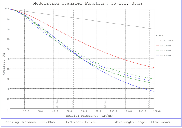
#35-181, 35mm, f/1.65 Cr Series Fixed Focal Length Lens, Modulated Transfer Function (MTF) Plot, 500mm Working Distance, f1.6
