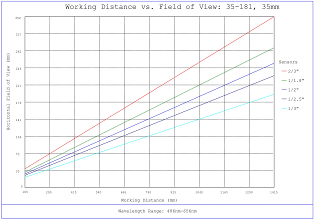
#35-181, 35mm, f/1.65 Cr Series Fixed Focal Length Lens, Working Distance versus Field of View Plot
