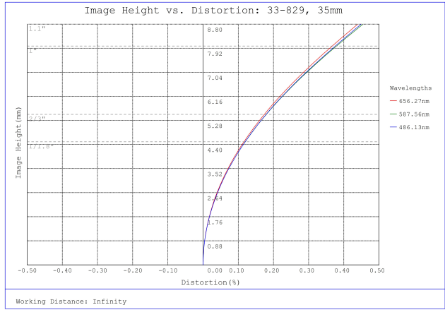
#33-829, 35mm f/2.0, HPI Series Fixed Focal Length Lens, Distortion Plot
