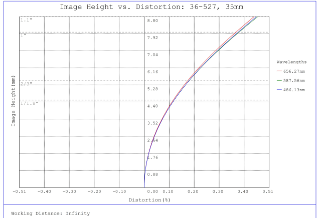
#36-527, 35mm f/2.8, HPr Series Fixed Focal Length Lens, Distortion Plot
