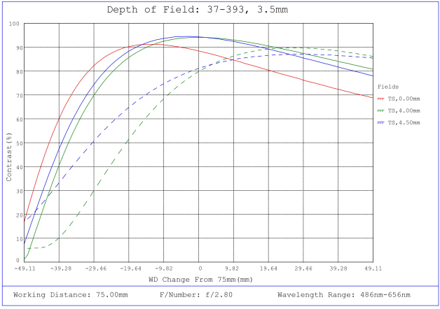
#37-393, 3.5mm, f/2.8 Cr Series Fixed Focal Length Lens, Depth of Field Plot, 75mm Working Distance, f2.8
