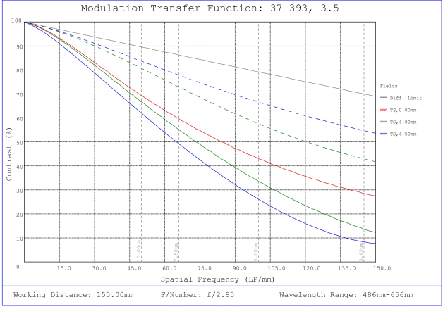
#37-393, 3.5mm, f/2.8 Cr Series Fixed Focal Length Lens, Modulated Transfer Function (MTF) Plot, 150mm Working Distance, f2.8
