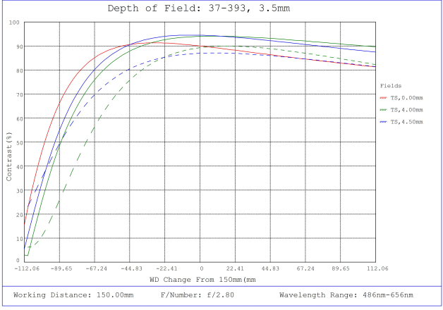
#37-393, 3.5mm, f/2.8 Cr Series Fixed Focal Length Lens, Depth of Field Plot, 150mm Working Distance, f2.8
