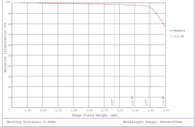
#37-393, 3.5mm, f/2.8 Cr Series Fixed Focal Length Lens, Relative Illumination Plot
