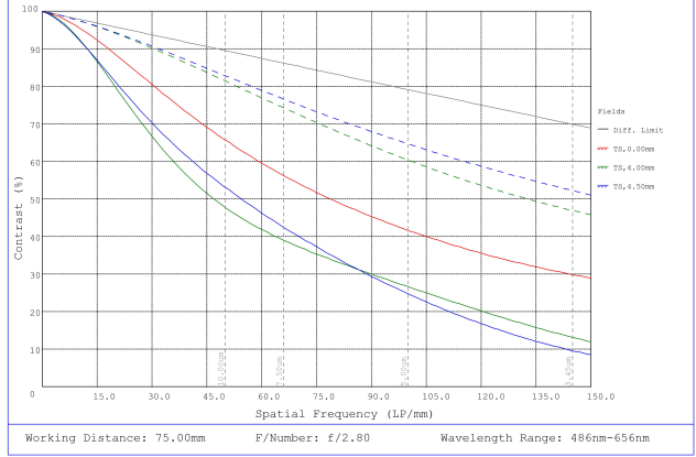
#37-393, 3.5mm, f/2.8 Cr Series Fixed Focal Length Lens, Modulated Transfer Function (MTF) Plot, 75mm Working Distance, f2.8
