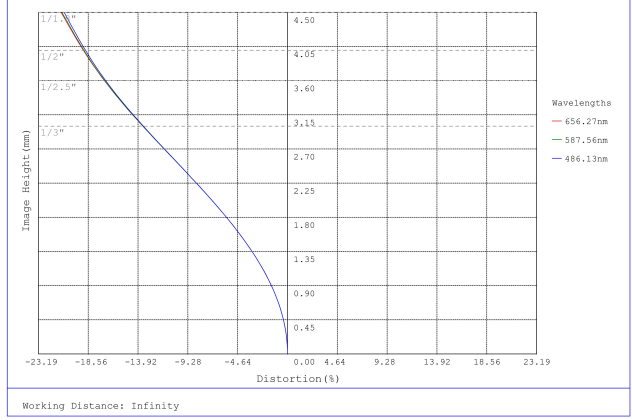
#37-393, 3.5mm, f/2.8 Cr Series Fixed Focal Length Lens, Distortion Plot
