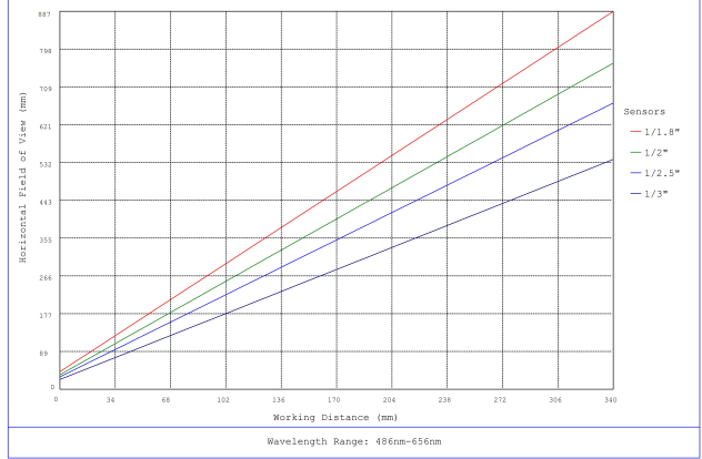
#37-393, 3.5mm, f/2.8 Cr Series Fixed Focal Length Lens, Working Distance versus Field of View Plot
