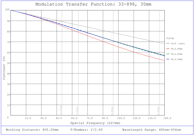
#33-898, 35mm f/2.8, UCI Series Fixed Focal Length Lens, Modulated Transfer Function (MTF) Plot, 400mm Working Distance, f2.8
