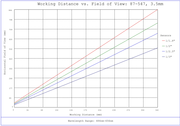
#87-547, 3.5mm, f/4 Ci Series Fixed Focal Length Lens, Working Distance versus Field of View Plot
