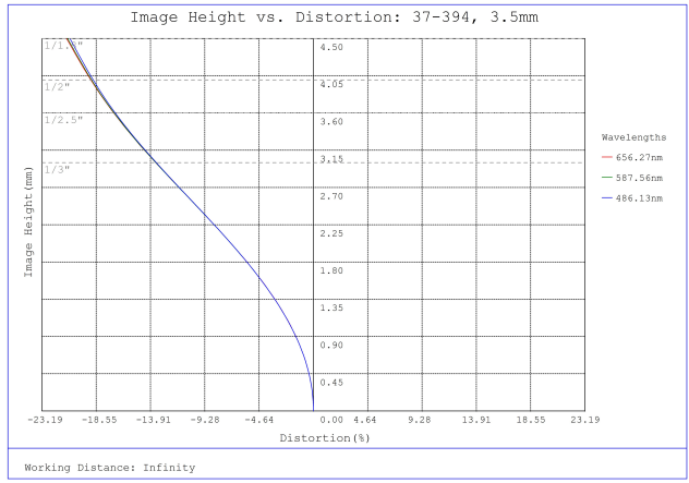
#37-394, 3.5mm, f/4 Cr Series Fixed Focal Length Lens, Distortion Plot
