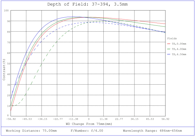
#37-394, 3.5mm, f/4 Cr Series Fixed Focal Length Lens, Depth of Field Plot, 75mm Working Distance, f4
