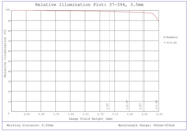
#37-394, 3.5mm, f/4 Cr Series Fixed Focal Length Lens, Relative Illumination Plot
