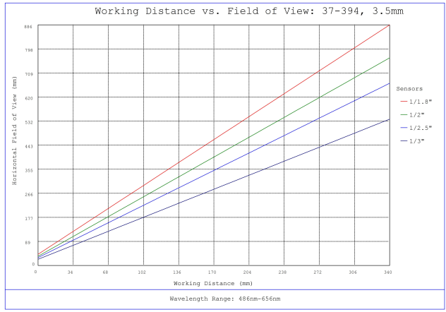
#37-394, 3.5mm, f/4 Cr Series Fixed Focal Length Lens, Working Distance versus Field of View Plot
