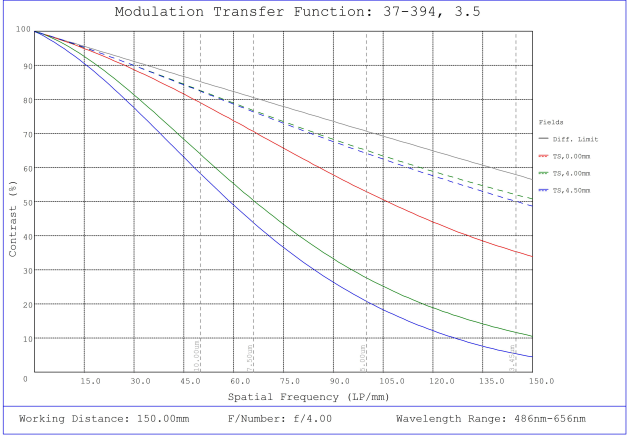
#37-394, 3.5mm, f/4 Cr Series Fixed Focal Length Lens, Modulated Transfer Function (MTF) Plot, 150mm Working Distance, f4
