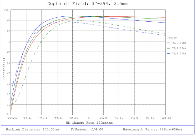
#37-394, 3.5mm, f/4 Cr Series Fixed Focal Length Lens, Depth of Field Plot, 150mm Working Distance, f4
