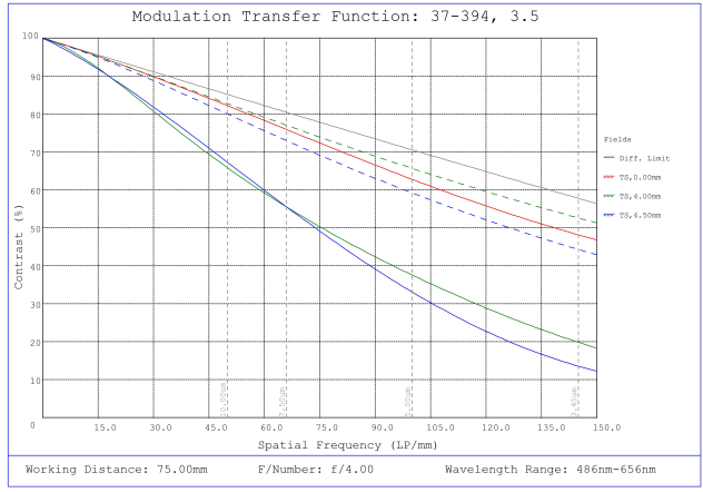
#37-394, 3.5mm, f/4 Cr Series Fixed Focal Length Lens, Modulated Transfer Function (MTF) Plot, 75mm Working Distance, f4
