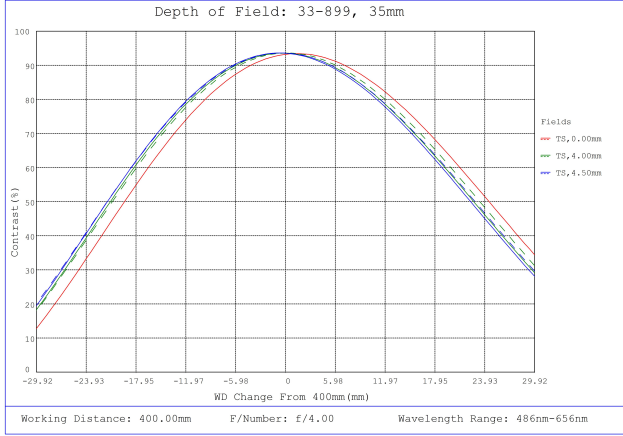
#33-899, 35mm f/4, UCI Series Fixed Focal Length Lens, Depth of Field Plot, 400mm Working Distance, f4
