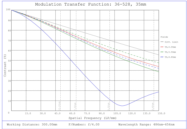
#36-528, 35mm f/4.0, HPr Series Fixed Focal Length Lens, Modulated Transfer Function (MTF) Plot, 300mm Working Distance, f4
