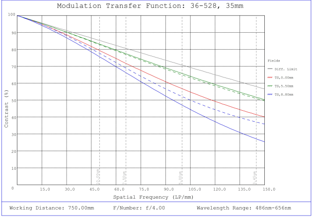
#36-528, 35mm f/4.0, HPr Series Fixed Focal Length Lens, Modulated Transfer Function (MTF) Plot, 750mm Working Distance, f4
