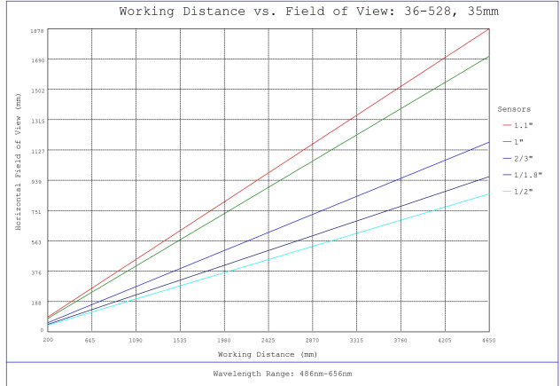
#36-528, 35mm f/4.0, HPr Series Fixed Focal Length Lens, Working Distance versus Field of View Plot
