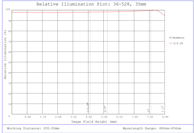
#36-528, 35mm f/4.0, HPr Series Fixed Focal Length Lens, Relative Illumination Plot
