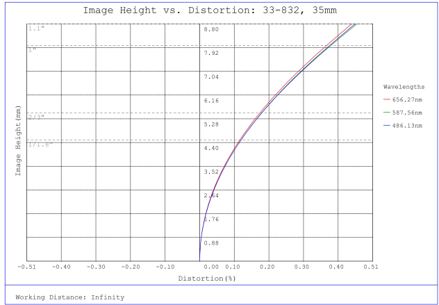
#33-832, 35mm f/5.6, HPI Series Fixed Focal Length Lens, Distortion Plot
