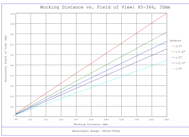
#85-366, 35mm, f/5.6 Ci Series Fixed Focal Length Lens, Working Distance versus Field of View Plot
