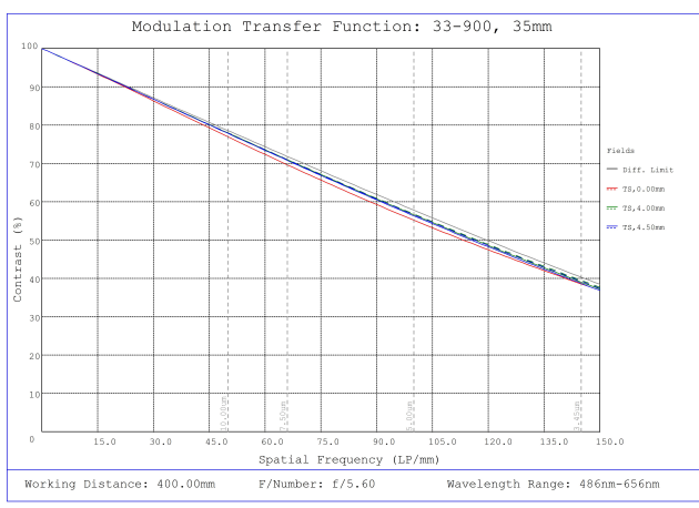
#33-900, 35mm f/5.6, UCi Series Fixed Focal Length Lens, Modulated Transfer Function (MTF) Plot, 400mm Working Distance, f5.6
