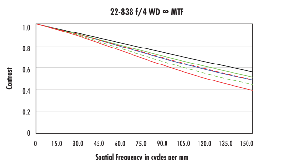
#22-838 - 35mm Focal Length, UAV Series Fixed Focal Length Lens, Modulated Transfer Function (MTF) Plot, Infinity Working Distance, f4
