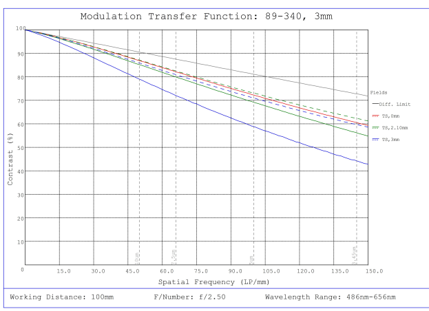
#20-055, 3mm FL f/2.5, IR-Cut Blue Series M12 Lens, Modulated Transfer Function (MTF) Plot, 100mm Working Distance, f2.5
