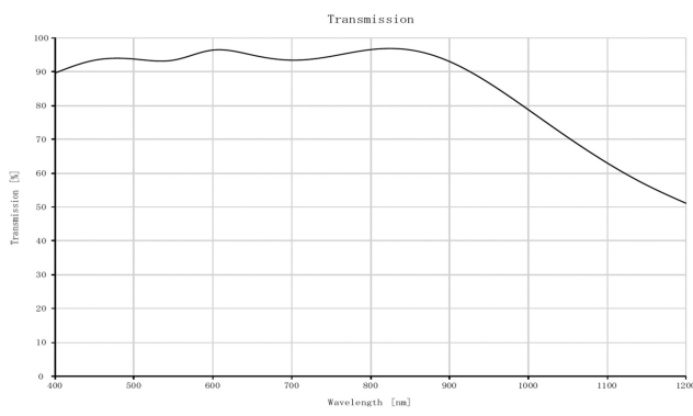
3mm FL, f/4, Low Distortion M12 Lens, Transmission Plot
