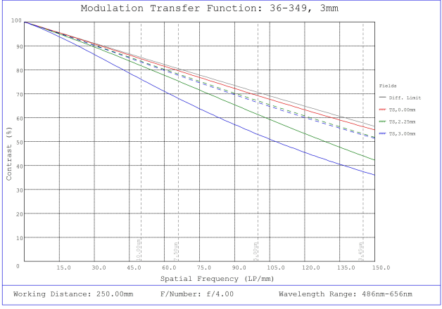
#36-349, 3mm FL f/4, Rugged Blue Series M12 Lens, Modulated Transfer Function (MTF) Plot, 250mm Working Distance, f4
