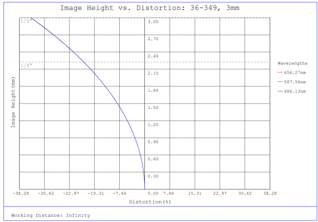
#36-349, 3mm FL f/4, Rugged Blue Series M12 Lens, Distortion Plot
