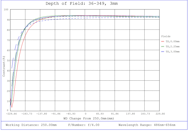
#36-349, 3mm FL f/4, Rugged Blue Series M12 Lens, Depth of Field Plot, 250mm Working Distance, f4
