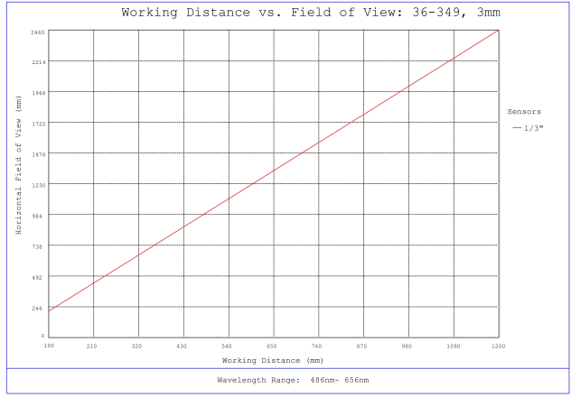
#36-349, 3mm FL f/4, Rugged Blue Series M12 Lens, Working Distance versus Field of View Plot
