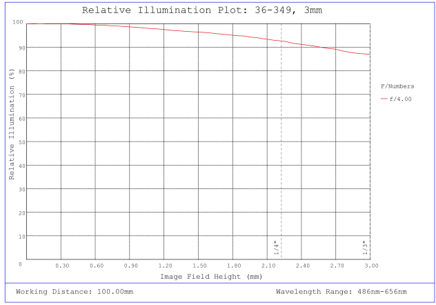
#36-349, 3mm FL f/4, Rugged Blue Series M12 Lens, Relative Illumination Plot
