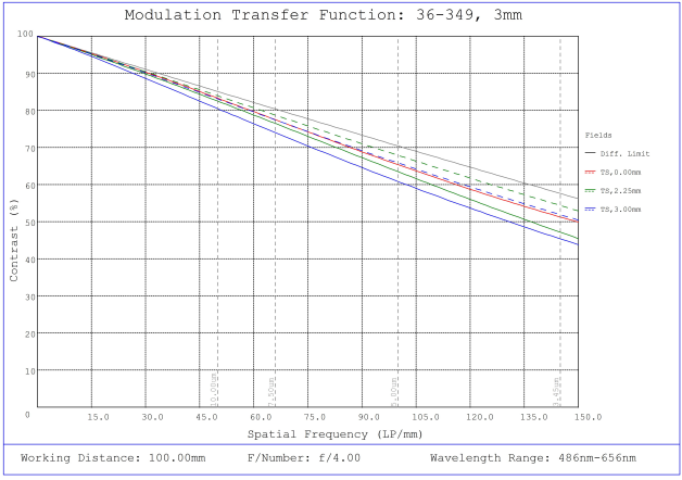
#36-349, 3mm FL f/4, Rugged Blue Series M12 Lens, Modulated Transfer Function (MTF) Plot, 100mm Working Distance, f4
