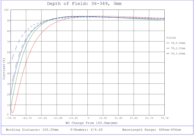
#36-349, 3mm FL f/4, Rugged Blue Series M12 Lens, Depth of Field Plot, 100mm Working Distance, f4
