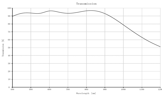
3mm FL, f/5.6, Low Distortion M12 Lens, Transmission Plot
