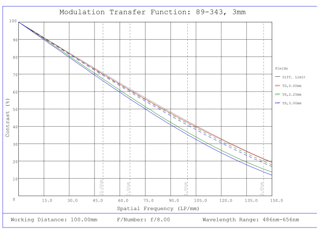
#89-343, 3mm FL f/8.0, Blue Series M12 Lens, Modulated Transfer Function (MTF) Plot, 100mm Working Distance, f8
