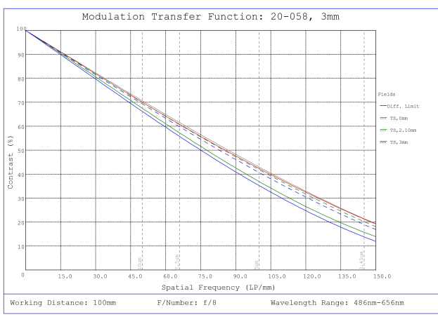
#20-058, 3mm FL f/8.0, IR-Cut Blue Series M12 Lens, Modulated Transfer Function (MTF) Plot, 100mm Working Distance, f8
