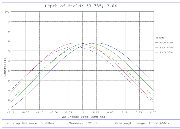
#63-735, 3X, 65mm WD CompactTL™ Telecentric Lens, Depth of Field Plot, 65mm Working Distance, f21.9
