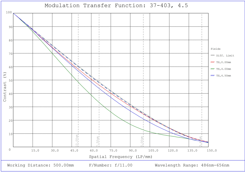
#37-403, 4.5mm, f/11 Cr Series Fixed Focal Length Lens, Modulated Transfer Function (MTF) Plot, 500mm Working Distance, f11
