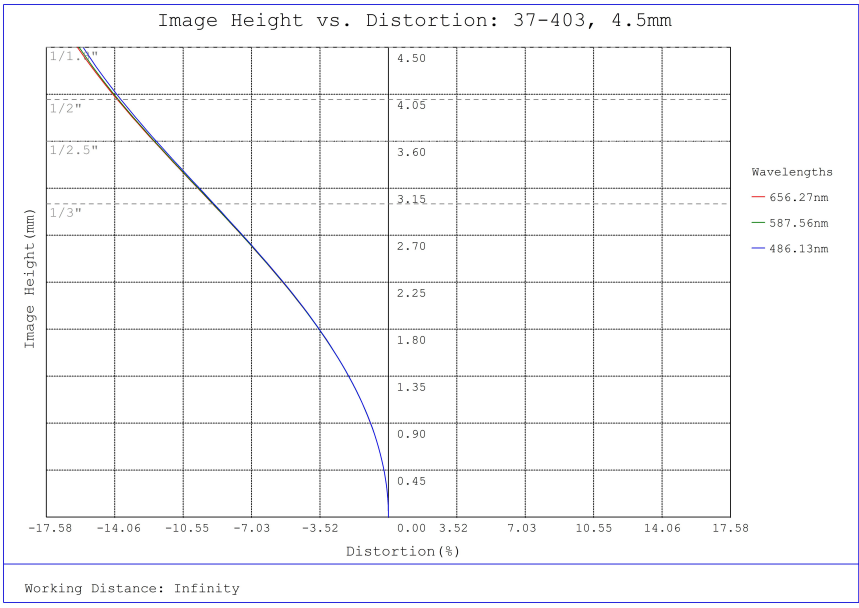
#37-403, 4.5mm, f/11 Cr Series Fixed Focal Length Lens, Distortion Plot
