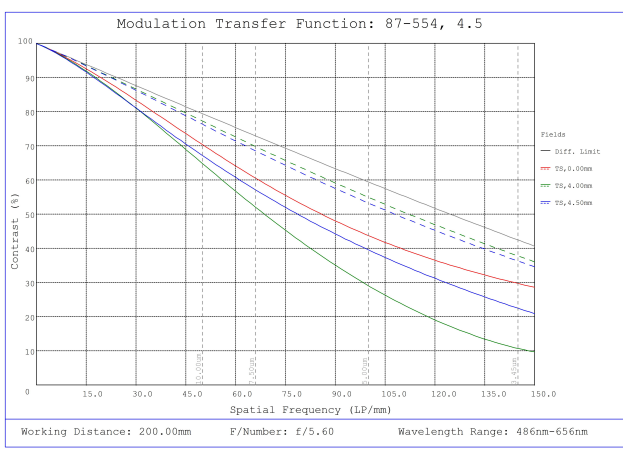
#87-554, 4.5mm, f/5.6 Ci Series Fixed Focal Length Lens, Modulated Transfer Function (MTF) Plot, 200mm Working Distance, f5.6
