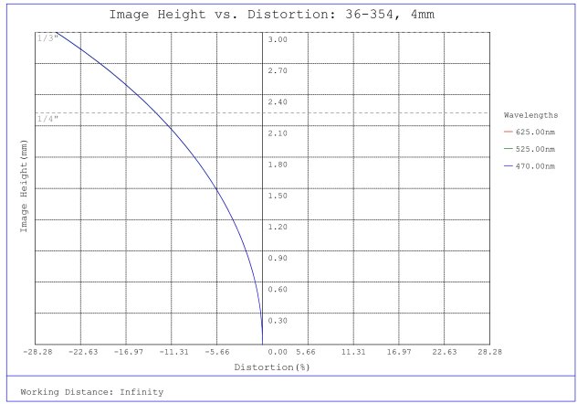
#36-354, 4mm FL f/5.6, Rugged Blue Series M12 Lens, Distortion Plot
