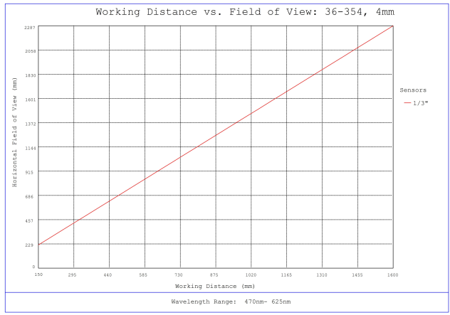
#36-354, 4mm FL f/5.6, Rugged Blue Series M12 Lens, Working Distance versus Field of View Plot
