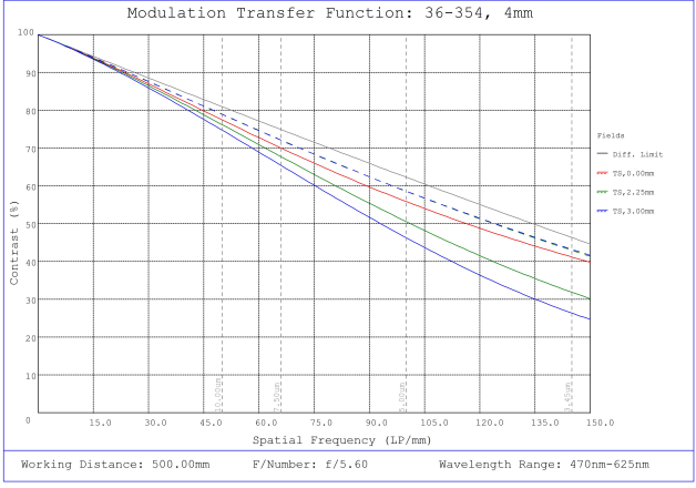
#36-354, 4mm FL f/5.6, Rugged Blue Series M12 Lens, Modulated Transfer Function (MTF) Plot, 500mm Working Distance, f5.6
