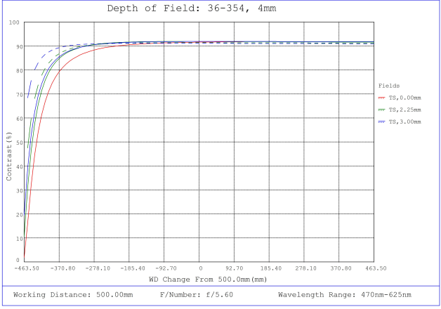
#36-354, 4mm FL f/5.6, Rugged Blue Series M12 Lens, Depth of Field Plot, 500mm Working Distance, f5.6
