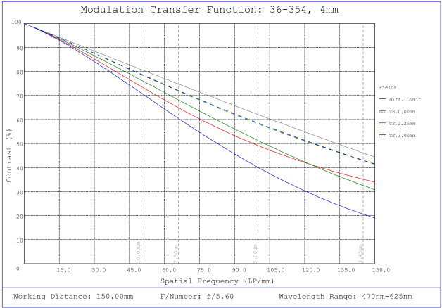
#36-354, 4mm FL f/5.6, Rugged Blue Series M12 Lens, Modulated Transfer Function (MTF) Plot, 150mm Working Distance, f5.6
