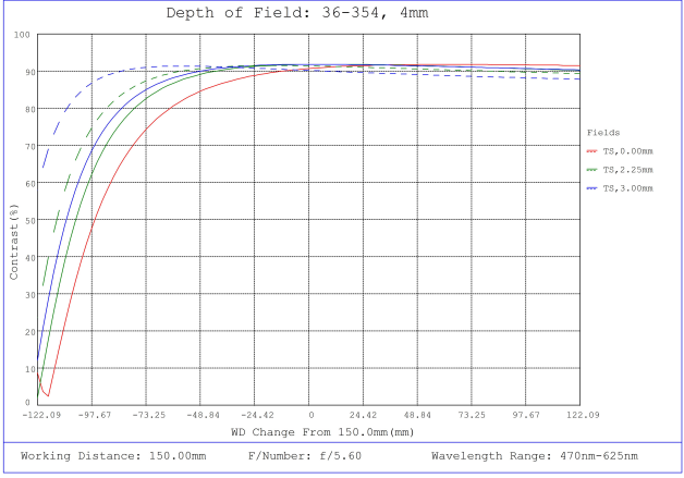
#36-354, 4mm FL f/5.6, Rugged Blue Series M12 Lens, Depth of Field Plot, 150mm Working Distance, f5.6
