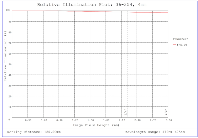
#36-354, 4mm FL f/5.6, Rugged Blue Series M12 Lens, Relative Illumination Plot
