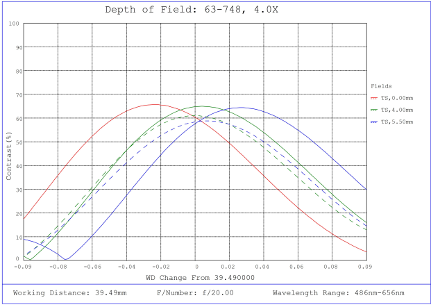
#63-748, 4X, 40mm WD CompactTL™ Telecentric Lens, Depth of Field Plot, 39mm Working Distance, f20
