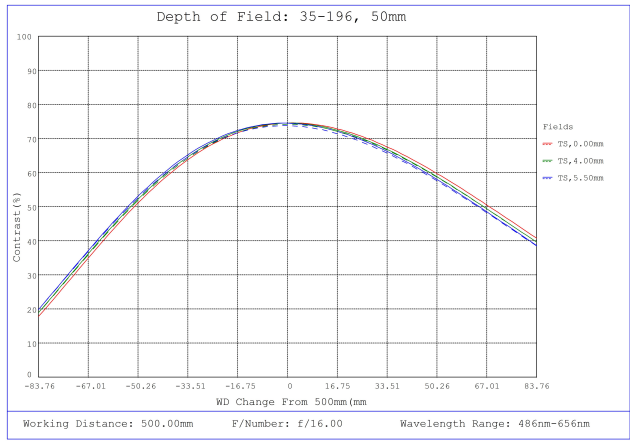
#35-196, 50mm, f/16 Cr Series Fixed Focal Length Lens, Depth of Field Plot, 500mm Working Distance, f16
