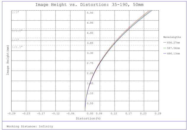
#35-190, 50mm, f/2.0 Cr Series Fixed Focal Length Lens, Distortion Plot
