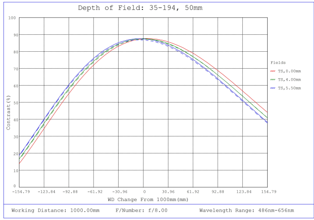
#35-194, 50mm, f/8.0 Cr Series Fixed Focal Length Lens, Depth of Field Plot, 1000mm Working Distance, f8
