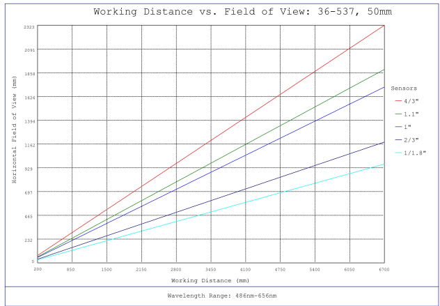
#36-537, 50mm f/11, HPr Series Fixed Focal Length Lens, Working Distance versus Field of View Plot
