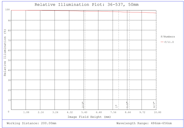
#36-537, 50mm f/11, HPr Series Fixed Focal Length Lens, Relative Illumination Plot
