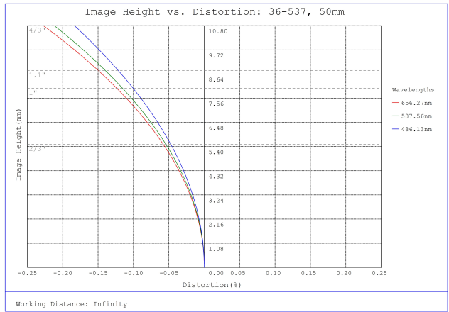
#36-537, 50mm f/11, HPr Series Fixed Focal Length Lens, Distortion Plot
