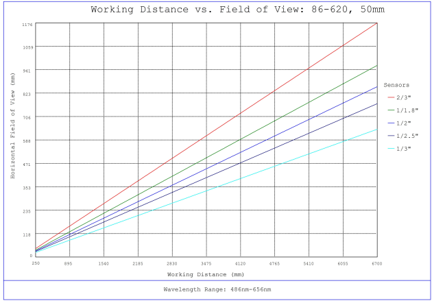
#86-620, 50mm, f/16.0 Ci Series Fixed Focal Length Lens, Working Distance versus Field of View Plot
