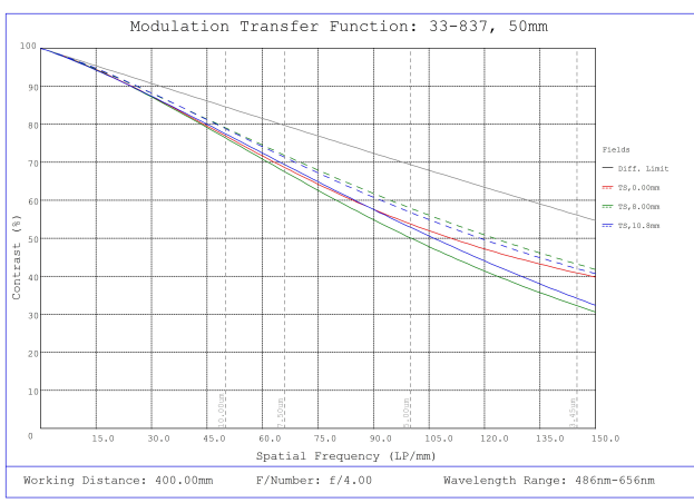
#33-837, 50mm f/4.0, HPI Series Fixed Focal Length Lens, Modulated Transfer Function (MTF) Plot, 400mm Working Distance, f4
