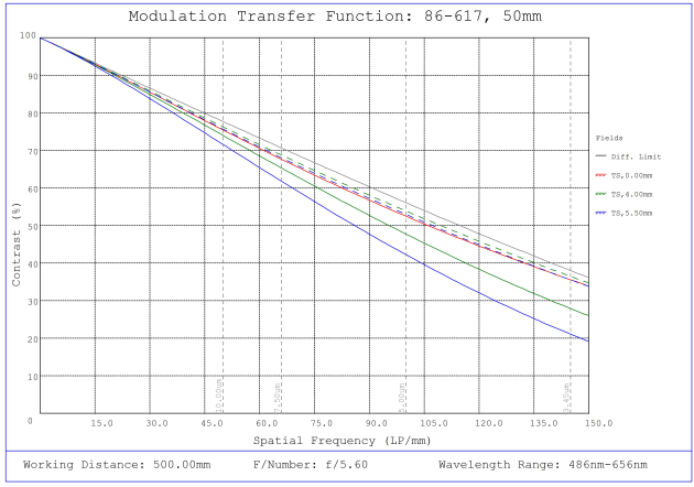
#86-617, 50mm, f/5.6 Ci Series Fixed Focal Length Lens, Modulated Transfer Function (MTF) Plot, 500mm Working Distance, f5.6
