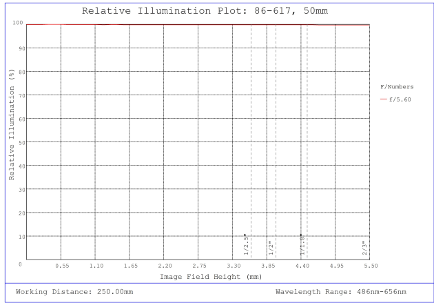
#86-617, 50mm, f/5.6 Ci Series Fixed Focal Length Lens, Relative Illumination Plot
