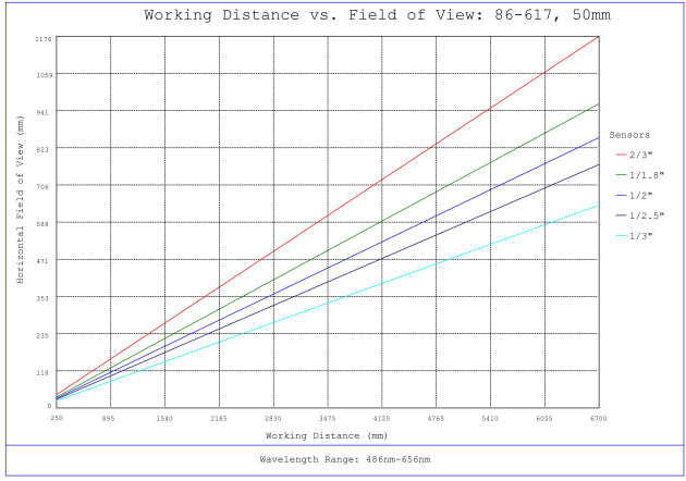
#86-617, 50mm, f/5.6 Ci Series Fixed Focal Length Lens, Working Distance versus Field of View Plot
