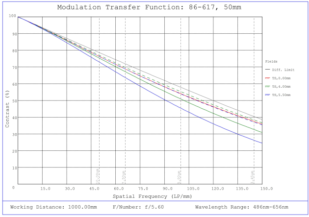
#86-617, 50mm, f/5.6 Ci Series Fixed Focal Length Lens, Modulated Transfer Function (MTF) Plot, 1000mm Working Distance, f5.6
