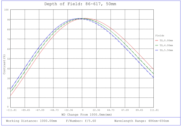
#86-617, 50mm, f/5.6 Ci Series Fixed Focal Length Lens, Depth of Field Plot, 1000mm Working Distance, f5.6
