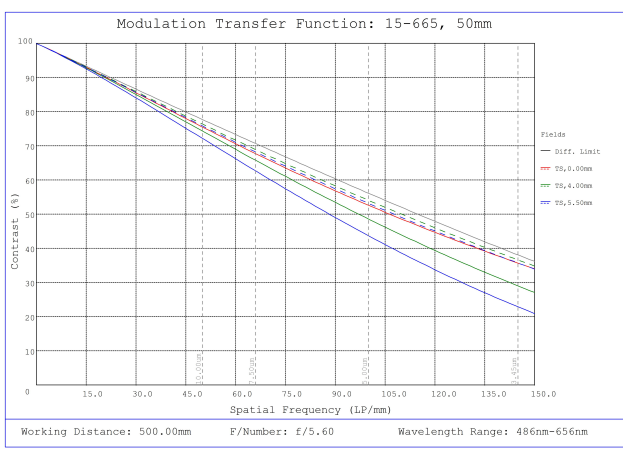
#15-665, 50mm, f/5.6 Sealed Cw Series Fixed Focal Length Lens, Modulated Transfer Function (MTF) Plot, 500mm Working Distance, f5.6
