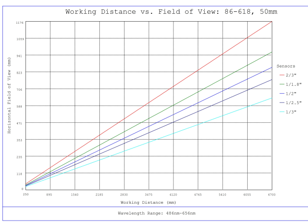
#86-618, 50mm, f/8.0 Ci Series Fixed Focal Length Lens, Working Distance versus Field of View Plot
