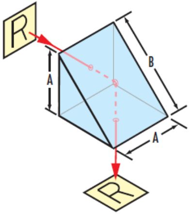
Image above shows light reflecting off the coated hypotenuse.
