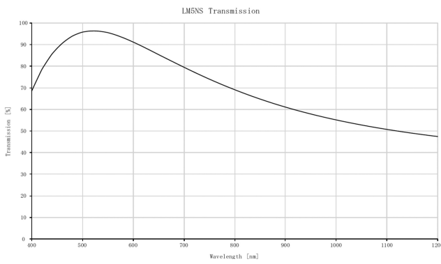
5mm FL, f/2.8, Low Distortion M12 Lens, Transmission Plot
