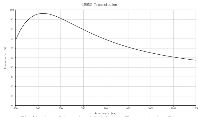
5mm FL, f/4, Low Distortion M12 Lens, Transmission Plot
