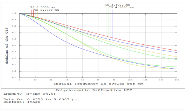
5mm FL, f/4, Low Distortion M12 Lens, MTF Plot
