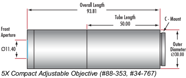
5X Compact Adjustable Objective (#88-353, #34-767)
