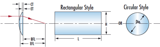
Circular And Rectangular Cylinder Lenses
