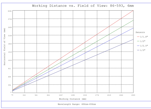
#86-593, 6mm, f/2.8 Ci Series Fixed Focal Length Lens, Working Distance versus Field of View Plot
