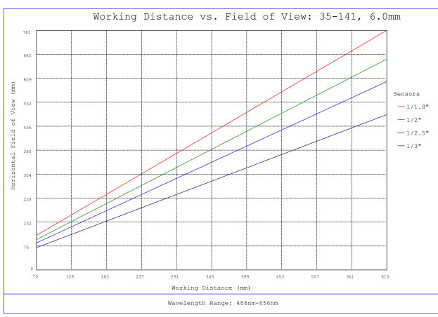
#35-141, 6mm, f/2.8 Cr Series Fixed Focal Length Lens, Working Distance versus Field of View Plot
