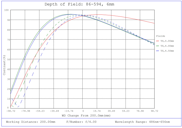
#86-594, 6mm, f/4 Ci Series Fixed Focal Length Lens, Depth of Field Plot, 200mm Working Distance, f4
