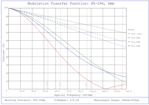
#86-594, 6mm, f/4 Ci Series Fixed Focal Length Lens, Modulated Transfer Function (MTF) Plot, 500mm Working Distance, f4
