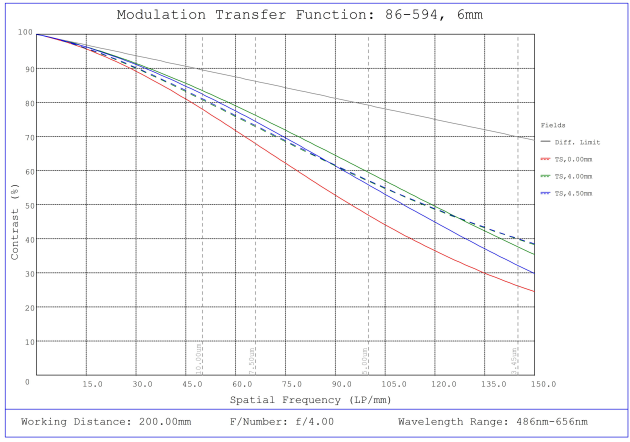
#86-594, 6mm, f/4 Ci Series Fixed Focal Length Lens, Modulated Transfer Function (MTF) Plot, 200mm Working Distance, f4
