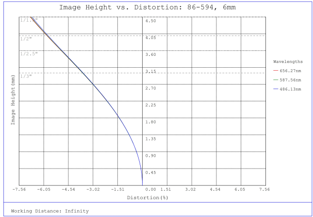
#86-594, 6mm, f/4 Ci Series Fixed Focal Length Lens, Distortion Plot
