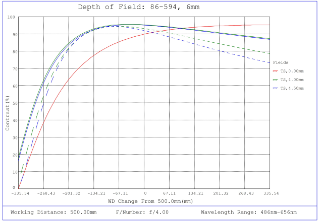
#86-594, 6mm, f/4 Ci Series Fixed Focal Length Lens, Depth of Field Plot, 500mm Working Distance, f4
