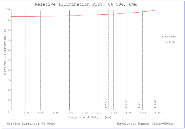
#86-594, 6mm, f/4 Ci Series Fixed Focal Length Lens, Relative Illumination Plot
