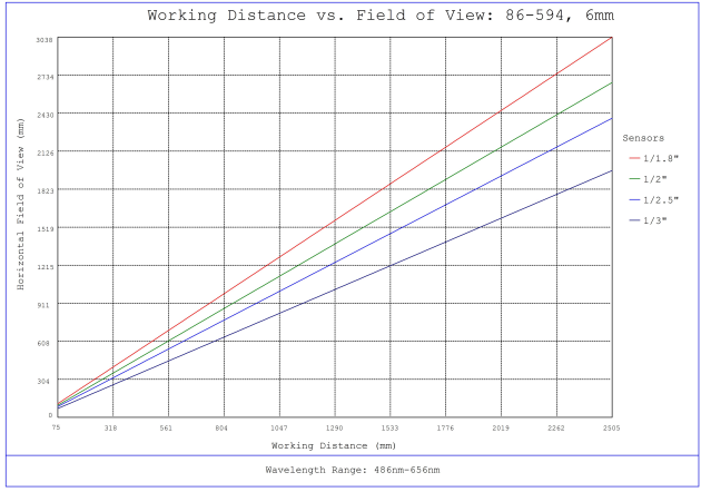
#86-594, 6mm, f/4 Ci Series Fixed Focal Length Lens, Working Distance versus Field of View Plot
