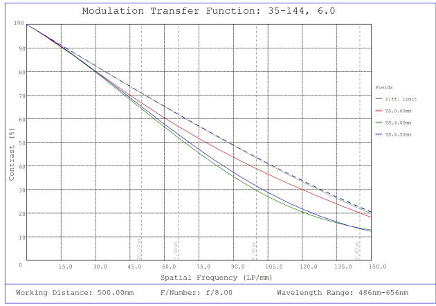
#35-144, 6mm, f/8 Cr Series Fixed Focal Length Lens, Modulated Transfer Function (MTF) Plot, 500mm Working Distance, f8
