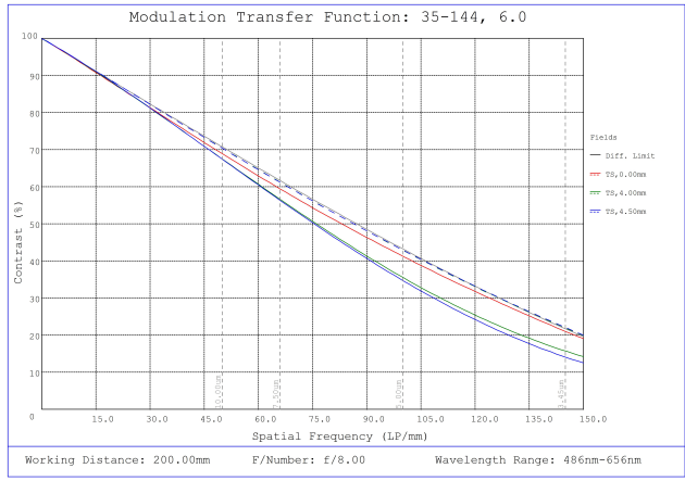
#35-144, 6mm, f/8 Cr Series Fixed Focal Length Lens, Modulated Transfer Function (MTF) Plot, 200mm Working Distance, f8
