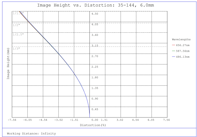
#35-144, 6mm, f/8 Cr Series Fixed Focal Length Lens, Distortion Plot
