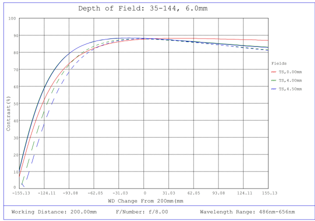
#35-144, 6mm, f/8 Cr Series Fixed Focal Length Lens, Depth of Field Plot, 200mm Working Distance, f8
