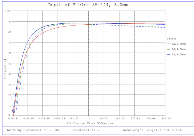
#35-144, 6mm, f/8 Cr Series Fixed Focal Length Lens, Depth of Field Plot, 500mm Working Distance, f8
