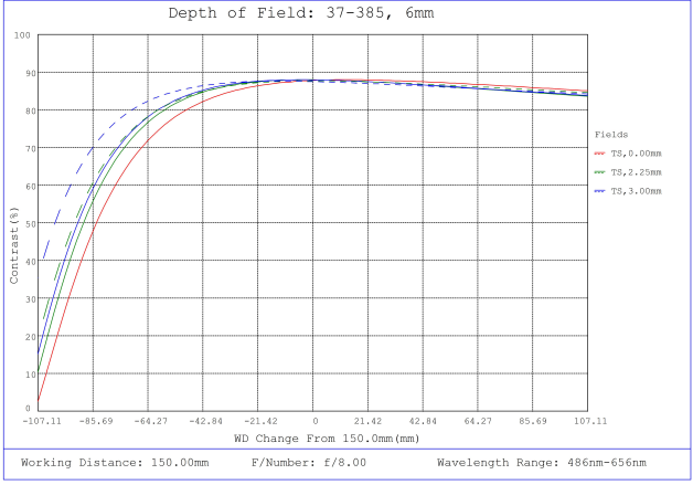
#37-385, 6mm FL f/8.0, Rugged Blue Series M12 Lens, Depth of Field Plot, 150mm Working Distance, f8
