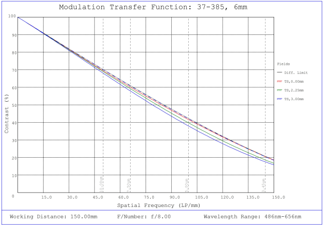
#37-385, 6mm FL f/8.0, Rugged Blue Series M12 Lens, Modulated Transfer Function (MTF) Plot, 150mm Working Distance, f8
