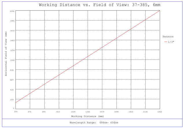
#37-385, 6mm FL f/8.0, Rugged Blue Series M12 Lens, Working Distance versus Field of View Plot
