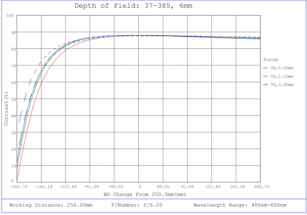
#37-385, 6mm FL f/8.0, Rugged Blue Series M12 Lens, Depth of Field Plot, 250mm Working Distance, f8
