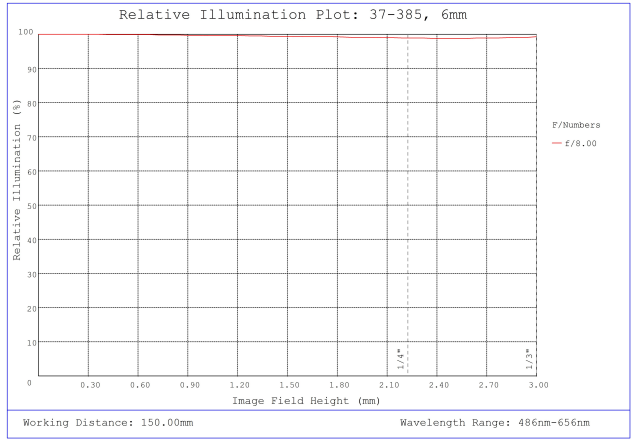
#37-385, 6mm FL f/8.0, Rugged Blue Series M12 Lens, Relative Illumination Plot
