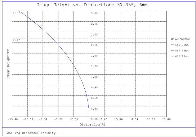
#37-385, 6mm FL f/8.0, Rugged Blue Series M12 Lens, Distortion Plot
