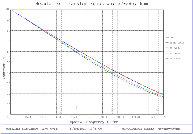
#37-385, 6mm FL f/8.0, Rugged Blue Series M12 Lens, Modulated Transfer Function (MTF) Plot, 250mm Working Distance, f8
